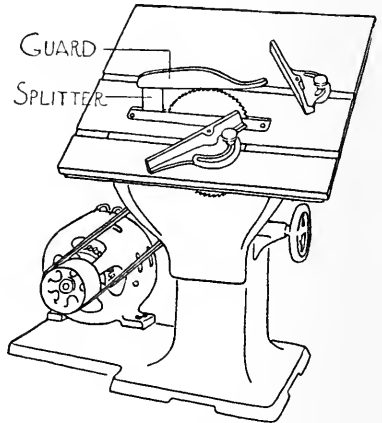
FIG. 157. SINGLE ARBOR CIRCULAR SAW.
